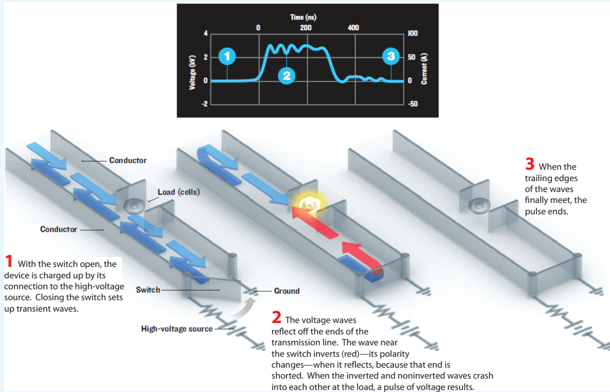
Figure TF4-3 High-voltage nanosecond pulse delivered to tumor cells via a transmission line. The cells to be shocked by the pulse sit in a break in one of the transmission-line conductors.
